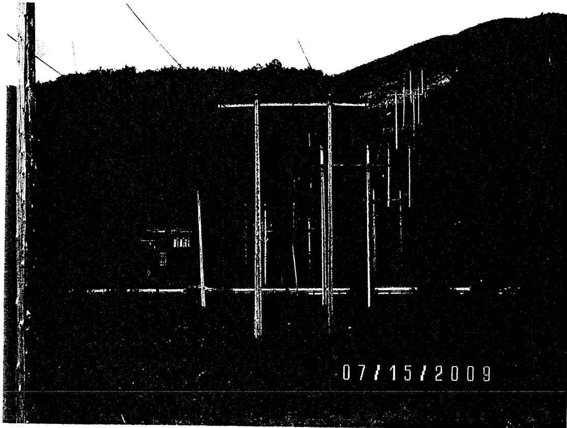
Figure IV-2 - Common H-Frame transmission line construction. (Photo courtesy of NHPUC)
