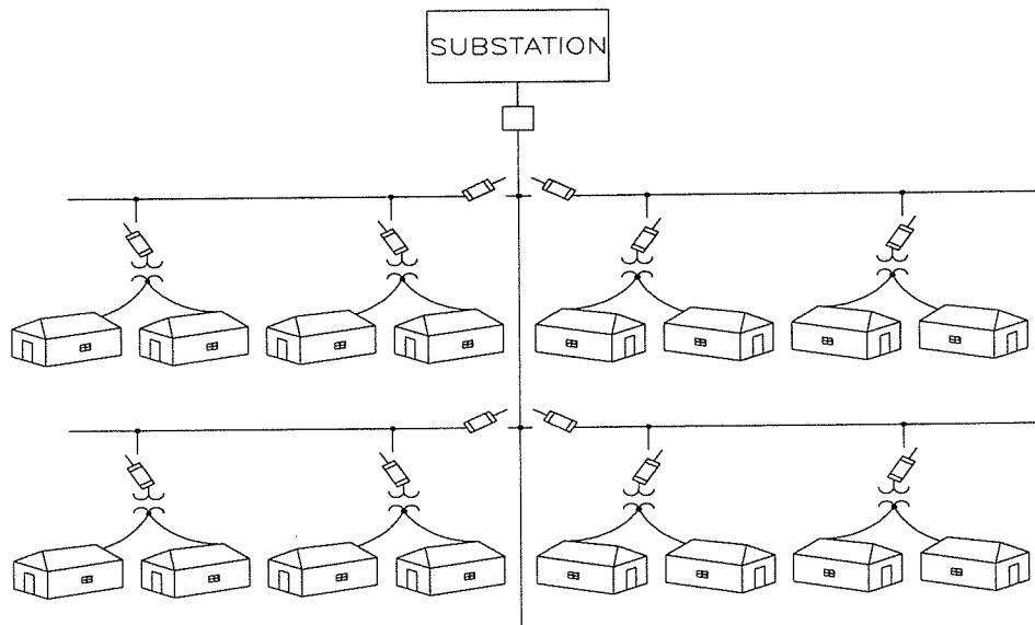
Figure B-6 - Typical radial distribution system.
