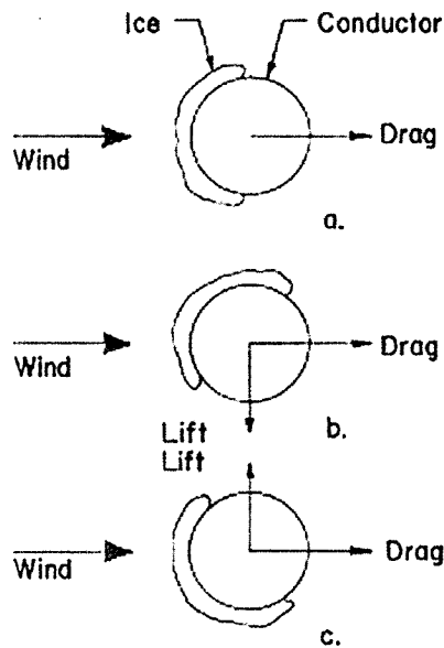
Figure F-7-Conditions causing galloping. 25
