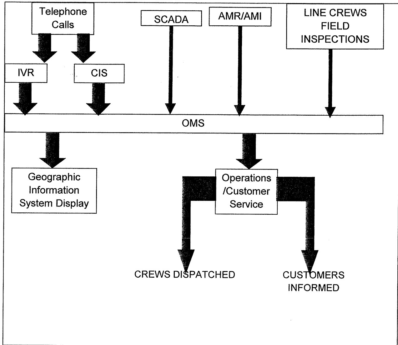
Figure G-1: OMS architecture.
