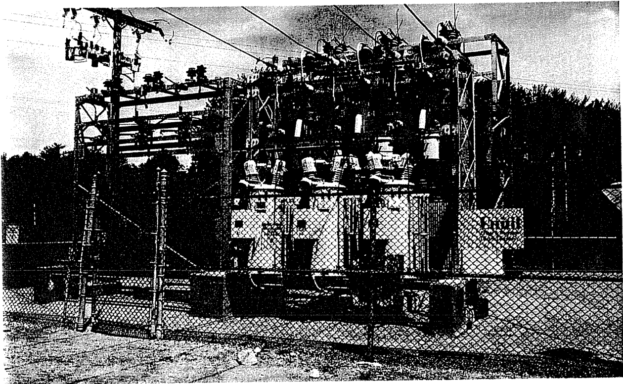
Figure IV-6 – 34.5kV to 13.8kV Unitil electric distribution substation located in East Kingston, New Hampshire. (Photo by NEI-Unitil System)
