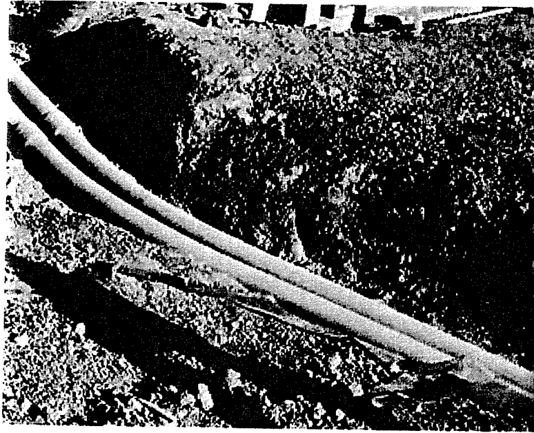
Figure B-5 - Conduit and Trench for Underground Distribution (Photo by NEI-Grand Prairie, Alberta)
