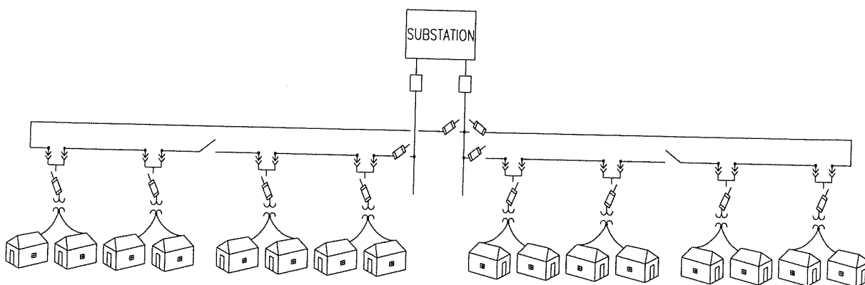
Figure B-7-Looped distribution system.
